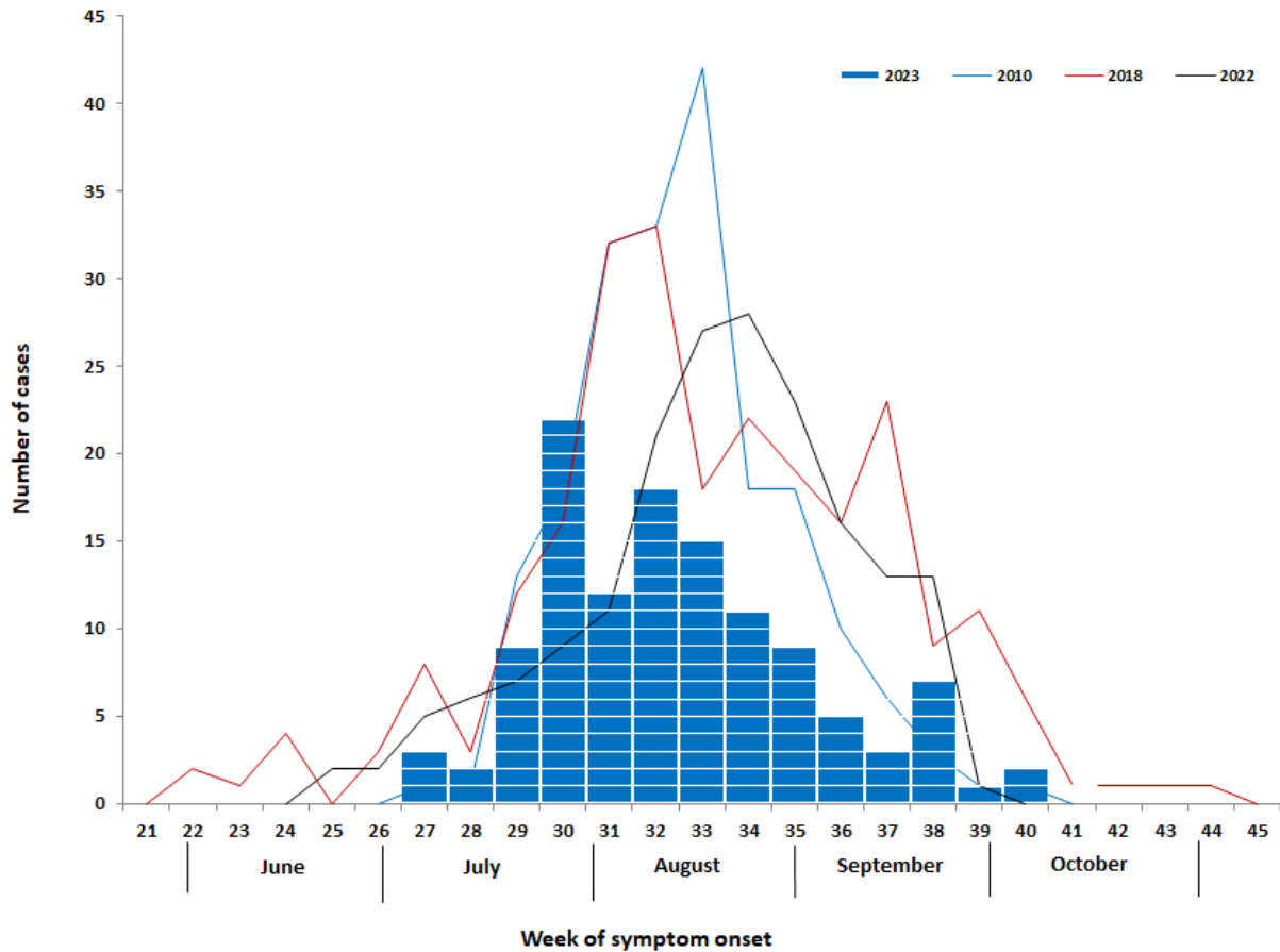
Figure 1. Number of reported WNNND cases (with central nervous system manifestations) by week of symptom onset, Greece, 2010, 2018, 2022 and 2023, up to 21/11/2023 (n=119) 1 .
