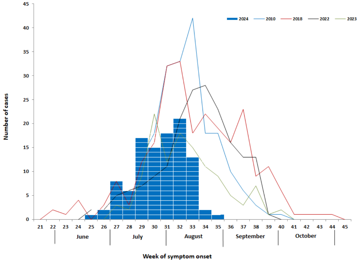
Figure 1. Number of locally acquired reported WNND cases (with central nervous system manifestations) by week of symptom onset, Greece, 2010, 2018, 2022, 2023 and 2024, up to 04/09/2024 (n=104) 1 .
