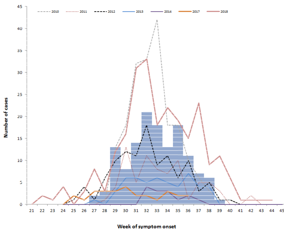
Figure 1. Number of laboratory diagnosed WNNND cases by week of symptom onset, Greece, 2010-2019 (until 03/10/2019).
