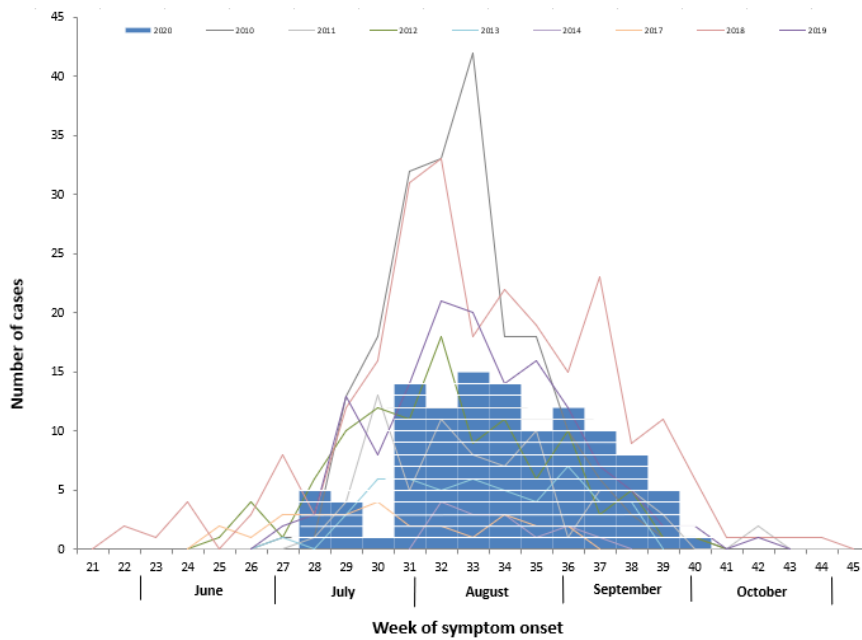
Figure 1. Number of laboratory diagnosed WNND cases by week of symptom onset, Greece, 2010-2020 (until 08/10/2020).
